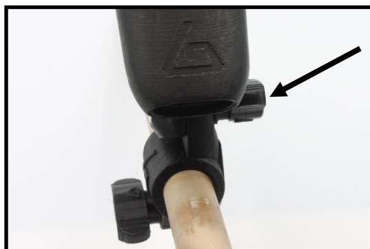
2.5. Add the magnetic support and the nut and tighten them with the butterfly, the magnetic support must be able to rotate
